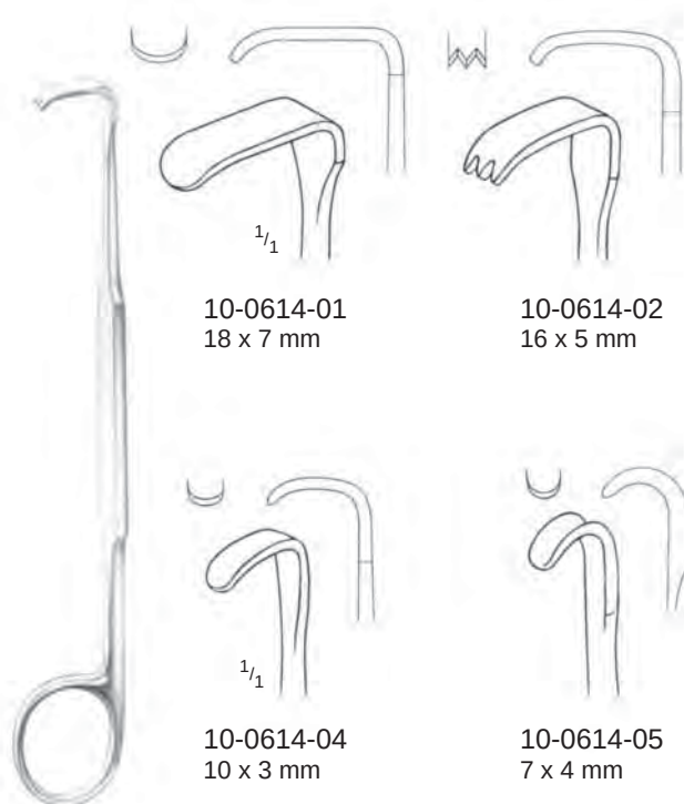
Meyerding Finger Retractors 18 cm/7" 10-0614-00 Satz/Set 6
